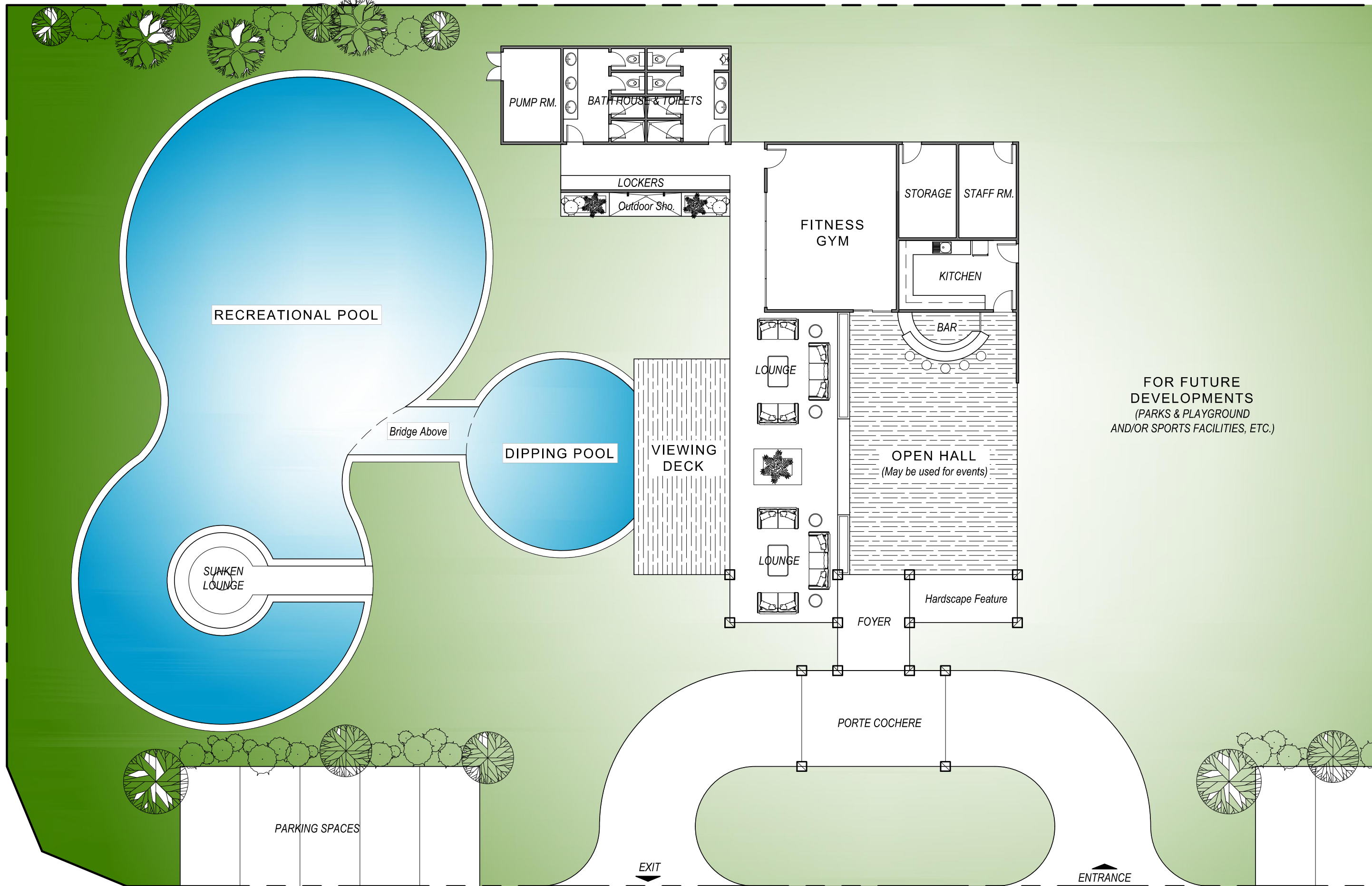
A CLUBHOUSE & SWIMMING POOL PLAN SCALE 1: 150 M
